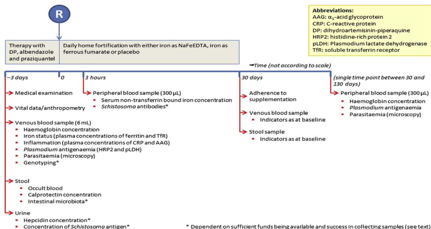
Fig. 2. Data collection timelines.
