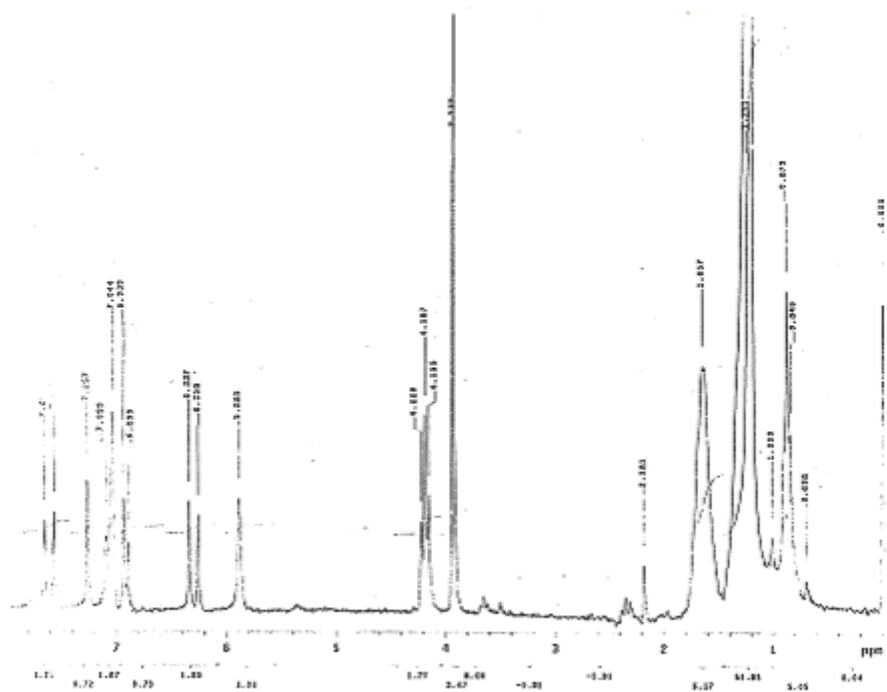
1 H NMR Spectrum of Erythrasinate (148)
