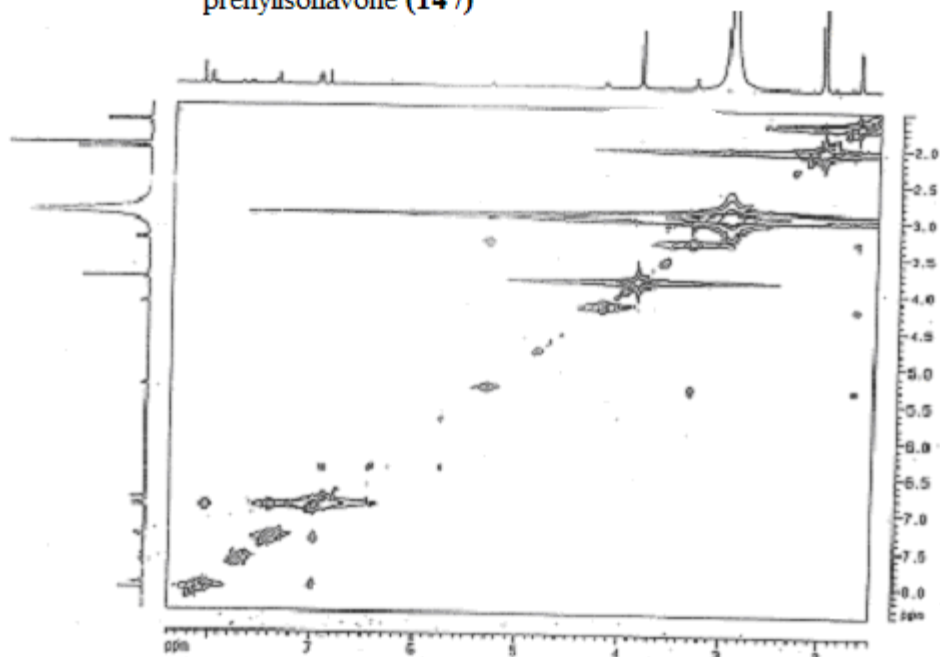
H-H COSY Spectrum of 7-hydroxy-4'-methoxy-3-prenylisoflavone (147)
