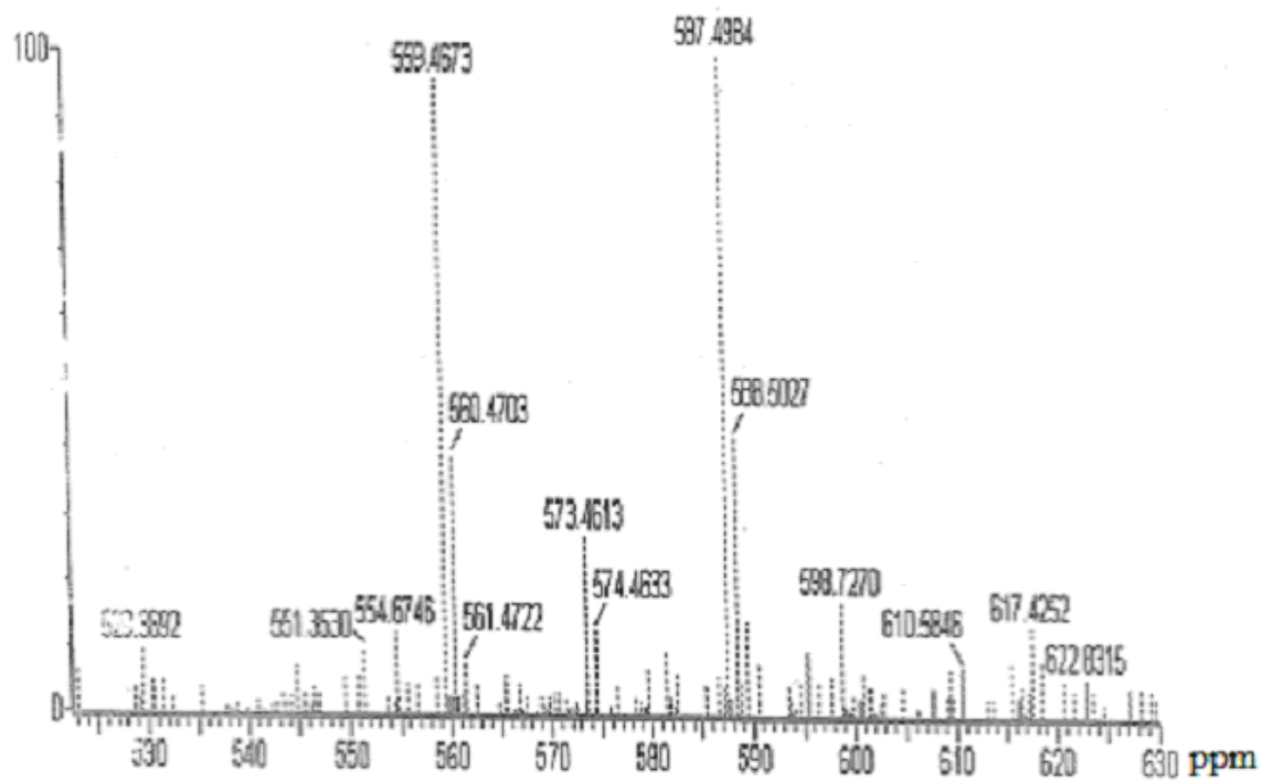
ESI-MS Spectrum of Erythrasinate ( 148 )
