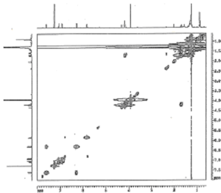
H-H COSY Spectrum of Erythrasinate ( 148 )
