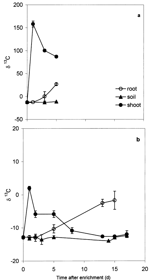
Figure 8. \delta^{13}C of plant samples obtained at varying time intervals after pulse labelling during wet (a) and dry (b) seasons. Sampling during wet conditions was discontinued due to rainfall and inaccessibility to the experimental site. Y-axes in the two figures are scaled differently to accommodate the large differences in ^{13}C signals and to improve clarity. Time zero represents unlabelled samples. Bars are \pm SE.
